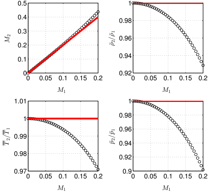
Figure 33: Evolution of the Mach number M_2 , \bar{\rho}_2/\bar{\rho}_1 , \bar{T}_2/\bar{T}_1 and \bar{p}_2/\bar{p}_1 with increasing M_1 predicted using the full equations (markers \circ ) and the simplified equations (solid lines). \bar{p}_1 = 1 \times 10^5 Pa, \bar{T}_1 = 300 K, \Theta = 0.5 .
