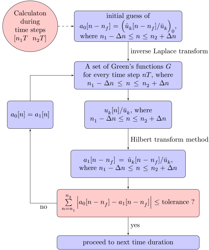
Figure 13: Flow chart of the “guess-and-comparison” method. Prediction of signal envelope in the time duration [n_1T \ n_2T] is carried out using the knowledge with a larger sample length n_1 - \Delta n \leq n \leq n_2 + \Delta n , where \Delta n denotes the number of additional samples padded at the two ends of raw signal.
