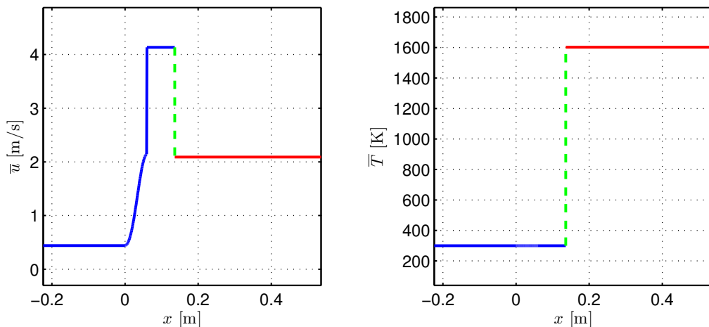
Figure 8: Plots of the mean velocity \bar{u} (left figure) and the mean temperature \bar{T} (right figure) in different sections.
