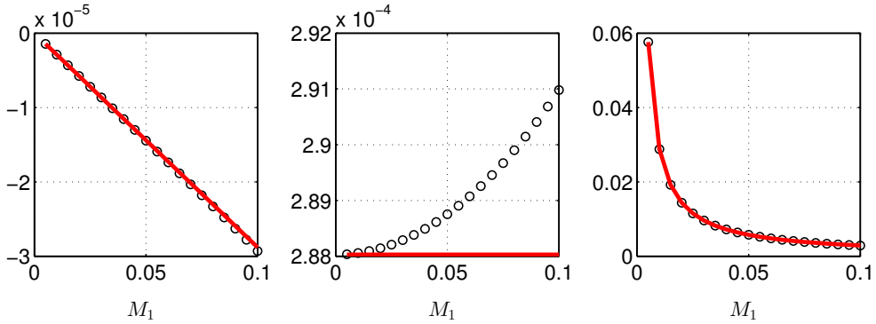
Figure 32: Evolution of the three elements of the 1 \times 3 array \mathbf{B}_2^{-1}\mathbf{A}\mathbf{r} and its simplification \mathbf{B}\mathbf{A}\mathbf{r} with increasing M_1 predicted using the full expression (markers \circ ) and the simplified expression (solid lines). \bar{p}_1 = 1 \times 10^5 Pa, \bar{T}_1 = 300 K, \bar{T}_2 = 1200 K, \Theta = 2 .
