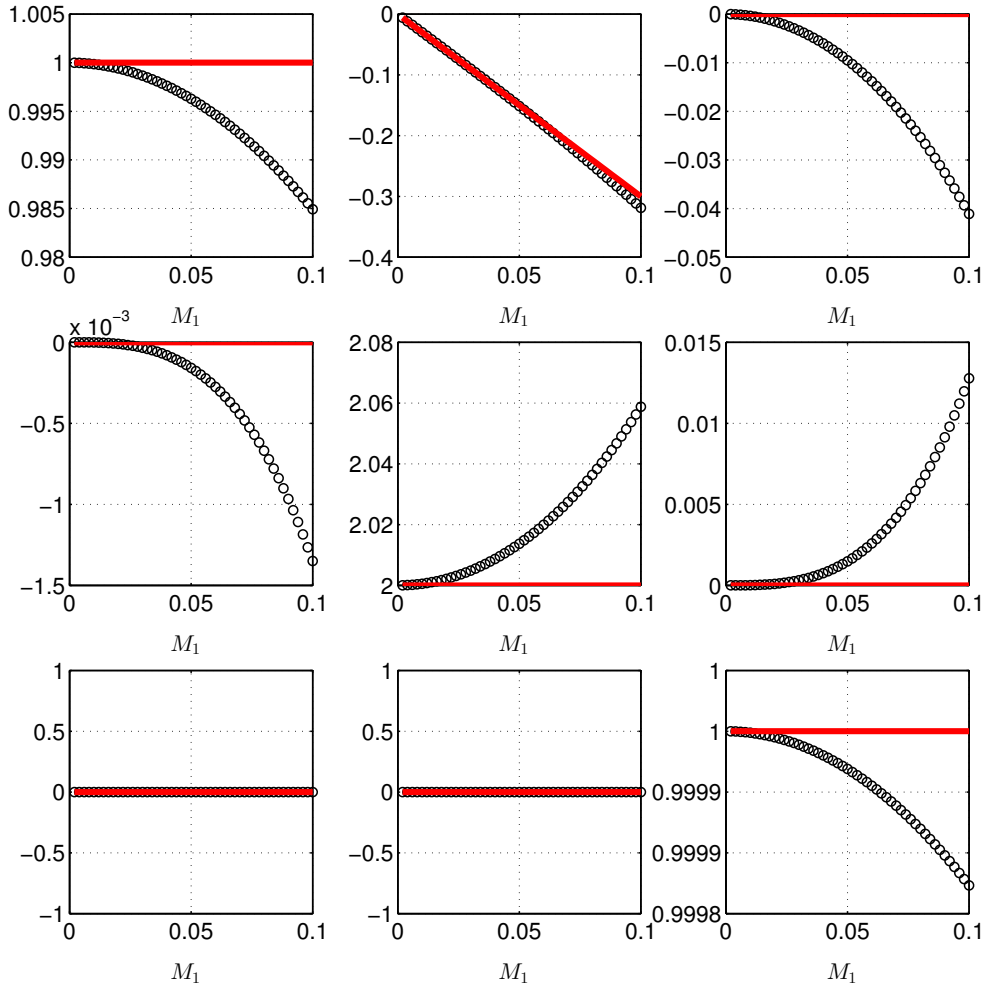
Figure 34: Evolution of the nine elements of the 3 \times 3 matrix \mathbf{B}_2^{-1}\mathbf{B}_1 and its simplification \mathbf{B}_3 with increasing M_1 predicted using the full expression (markers \circ ) and the simplified expression (solid lines). \bar{p}_1 = 1 \times 10^5 Pa, \bar{T}_1 = 300 K, \Theta = 0.5 .
