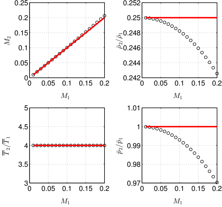
Figure 30: Evolution of the Mach number M_2 , \bar{\rho}_2/\bar{\rho}_1 , \bar{T}_2/\bar{T}_1 and \bar{p}_2/\bar{p}_1 with increasing M_1 predicted using the full equations (markers \circ ) and the simplified equations (solid lines). \bar{p}_1 = 1 \times 10^5 Pa, \bar{T}_1 = 300 K, \bar{T}_2 = 1200 K, \Theta = 2 .
