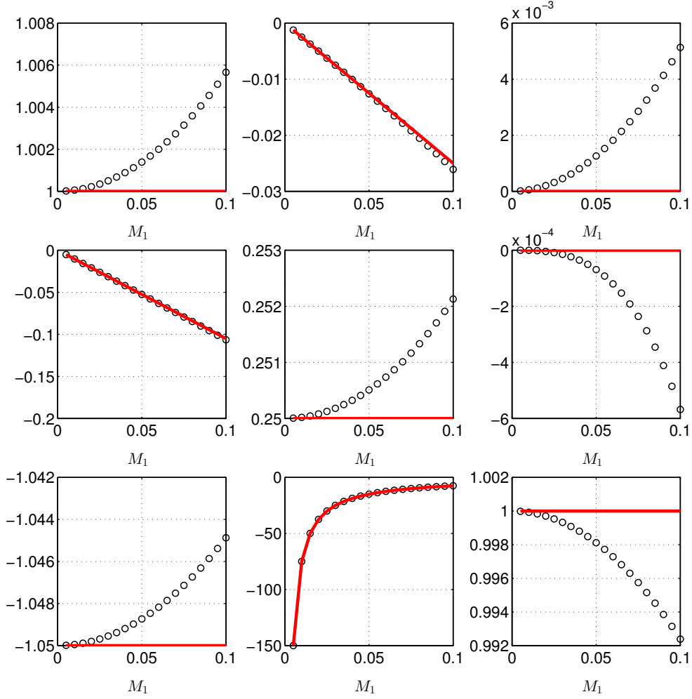
Figure 31: Evolution of the nine elements of the 3 \times 3 matrix \mathbf{B}_2^{-1}\mathbf{B}_1 and its simplification \mathbf{B}_3 with increasing M_1 predicted using the full expression (markers \circ ) and the simplified expression (solid lines). \bar{p}_1 = 1 \times 10^5 Pa, \bar{T}_1 = 300 K, \bar{T}_2 = 1200 K, \Theta = 2 .
